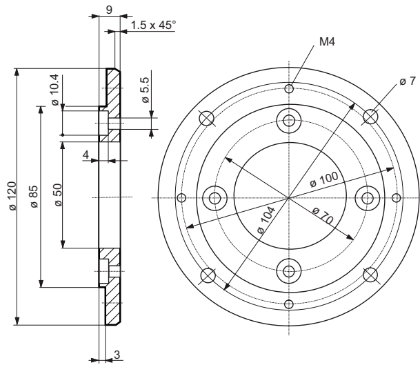
Mounting flange MF 121
