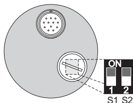
DIP switches behind screw cap on the rear side of the encoder
