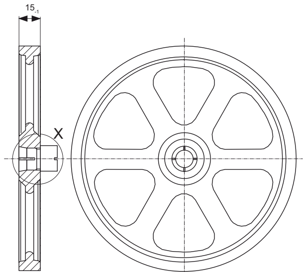
MRG 500 Operating temperature (rubber)
